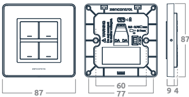
To suit 60 mm wall mount Dimensions 87 / 87 / 13 mm Mounting centres 60 mm
