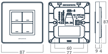
To suit 60 mm wall mount Dimensions 87 / 87 / 13 mm Mounting centres 60 mm
