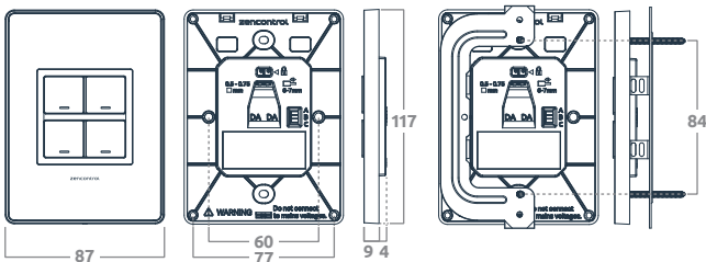
To suit 84 mm wall mount Dimensions 87 / 117 / 13 mm Mounting centres 84 mm
