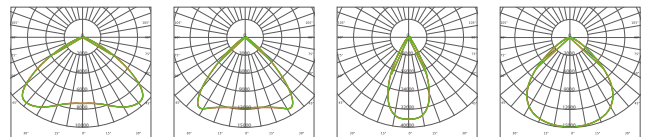
Polar drawing
